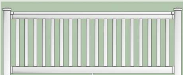
VR6T/8-3 • VRT6/8-42 3' or 42" Height Traditional Spindle 1 1/2" x 1 1/2" T-Rail Top & 2" x 3 1/2" Bottom Rail 6' or 8' Wide
